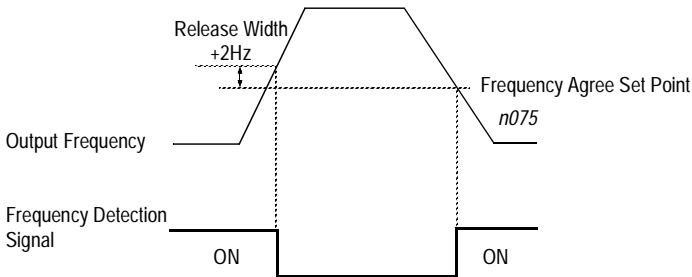
Figure 26 Frequency Agree Set Point Example (Fout ≤ Frequency Agree Set Point)
