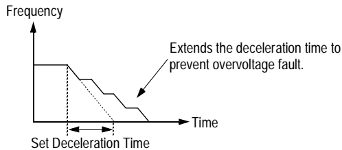
Figure 22 Stall Prevention During Deceleration
