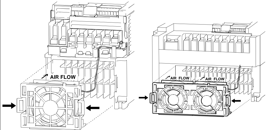
FR-F540J-1.5K~3.7K-CH
