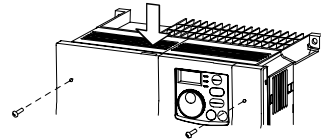
FR-F540J-5.5K~15K-CH
