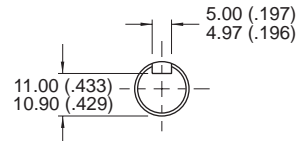
KEYWAY DETAIL
