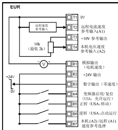
图 6-1 Pr05 = AI.AU
